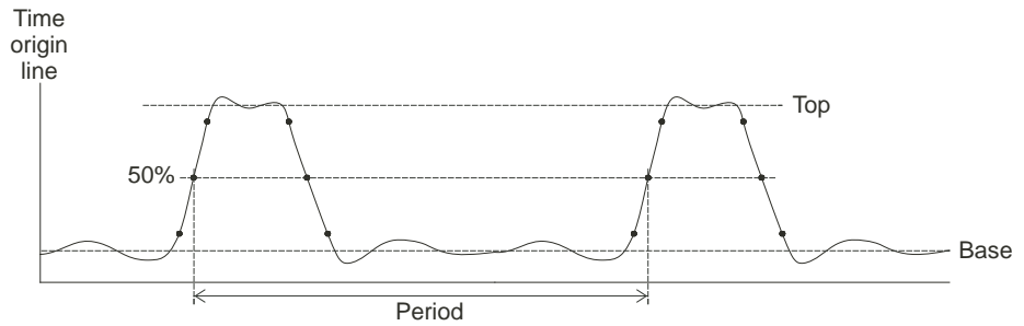
Figure 41 Period and Frequency Measurements
